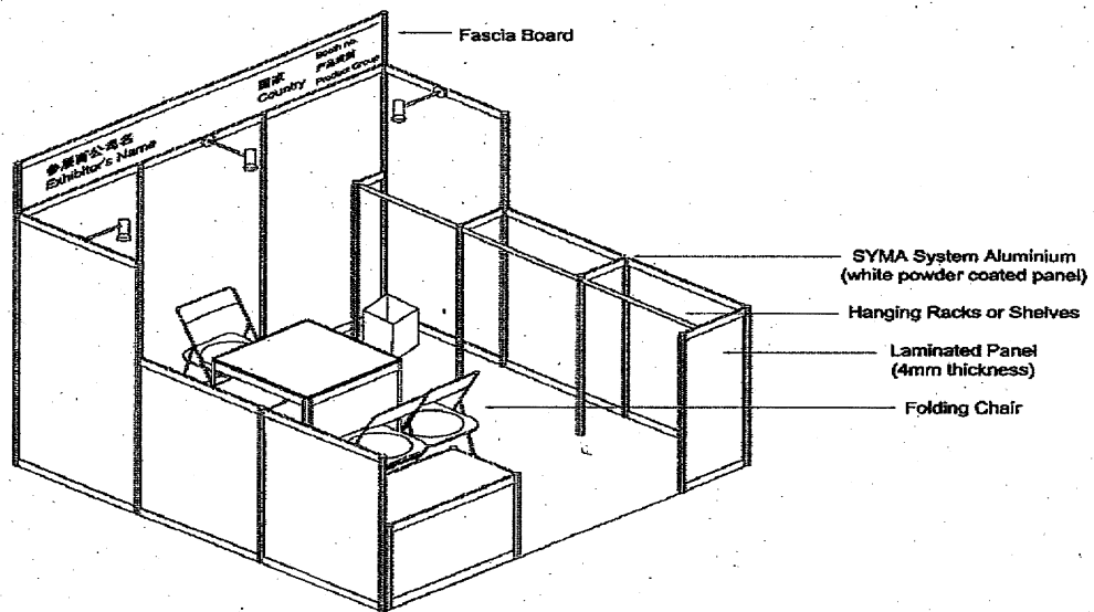
ISOMETRIC
